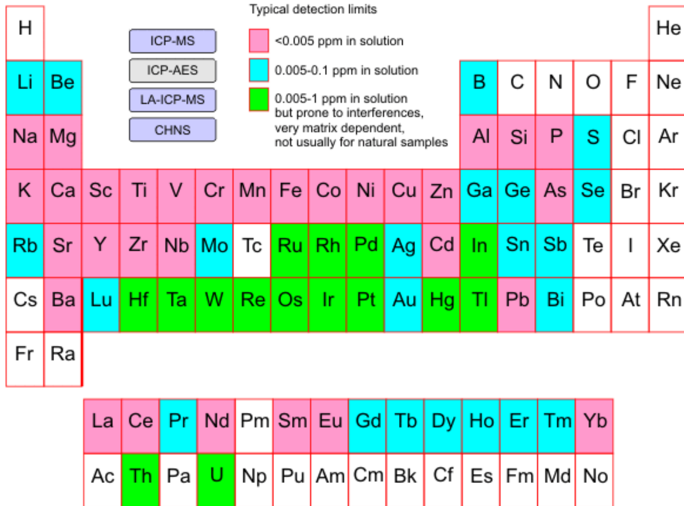
Periodic Table showing elemental range and typical detection limits for ICP-AES
