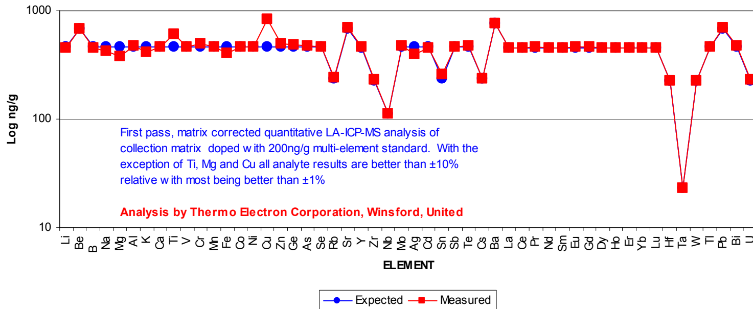
EXPECTED Vs MEASURED CONCENTRATION Matrix Doped With 200ng/g Multi-element Standard
