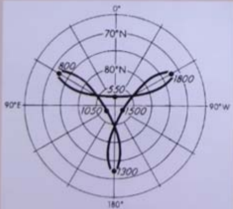
Fig. 1 Model of quasi-hypotrochoid motion of the geomagnetic dipole axis during historic times. Numbers on the curve represent dates in yr AD (after N. Kawai and K. Hirooka's).
